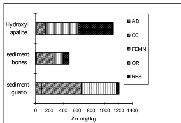
Fig. 3 Zinc concentrations in the cave sediment fractions, hydroxylapatite= hydroxylapatite crusts on flowstone.
